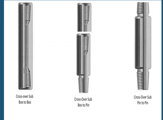
Crossover Subs
